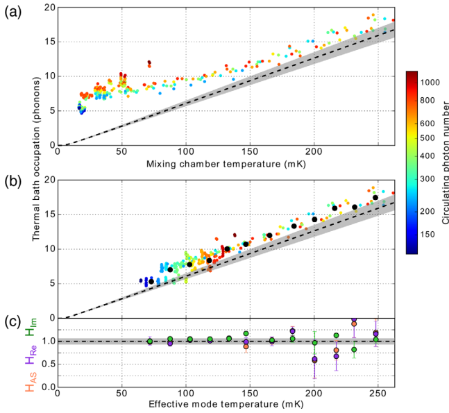
FIG. 3. Thermal and quantum fluctuations of the acoustic mode. (a) The mean phonon number n_{\text{th}} associated with the acoustic mode's bath temperature plotted vs T_{\text{MC}} . (b) The same measurements of n_{\text{th}} as in (a) but plotted as a function of T_{\text{eff}} , the effective device temperature calculated in the Supplemental Material [31]. The color of each marker encodes n_{\text{circ}} , the intracavity photon number. The black points are obtained by averaging data in 15 mK bins. In both (a) and (b), the dashed lines show the expected behavior n_{\text{th}} = 1/(e^{\hbar\omega_{\text{ac}}/k_B T} - 1) , while the gray area represents the systematic uncertainty resulting from the calibration of the heterodyne signal (Supplemental Material [31]). (c) Three measures of the quantum features plotted as a function of T_{\text{eff}} . The dashed line is the prediction of quantum optomechanics theory; the gray area shows the systematic uncertainty resulting from the calibration of the heterodyne signal. Each data point is produced from data and fits similar to Fig. 2 (averaged over 15 mK bins). Error bars indicate the statistical uncertainty in these fits.
